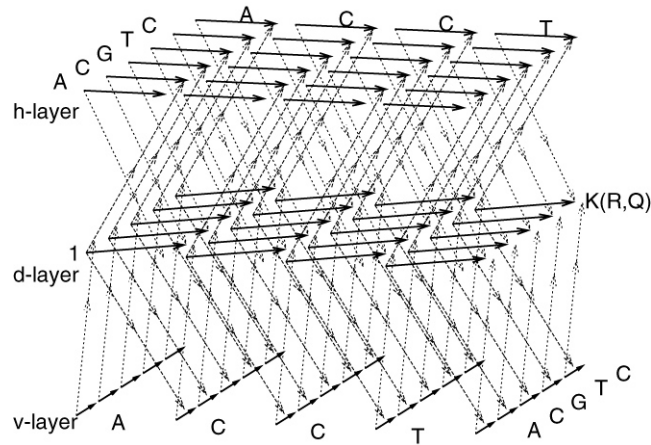
Fig. 3. '3D' version of sequence alignment, which accounts for affine gaps.
