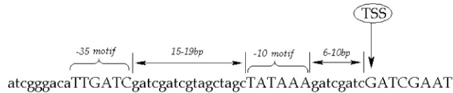
Fig. 1. Prokaryotic \sigma^{70} promoter region with TSS, ‘-10’ and ‘-35’ binding motifs and two spacers.
