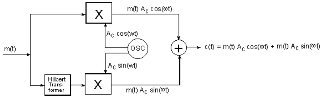
Figure 14 - SSB Modulator using the Phasing method
