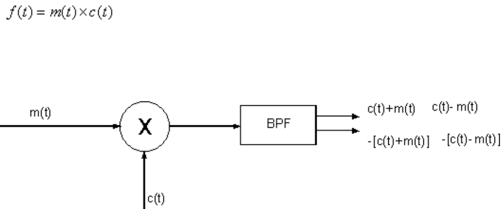
Figure 3 - A Product Modulator
