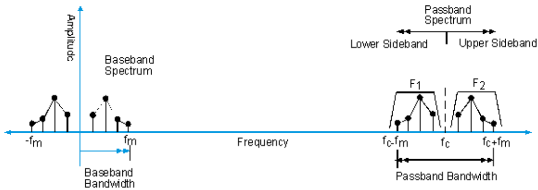
Figure 7 - Filter passband to for the upper and lower side-band as separate signals.
