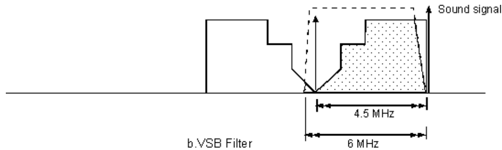
Figure 16b - Vestigial Filter
