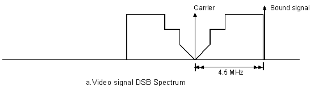
Figure 16a - Video Signal bandwidth
