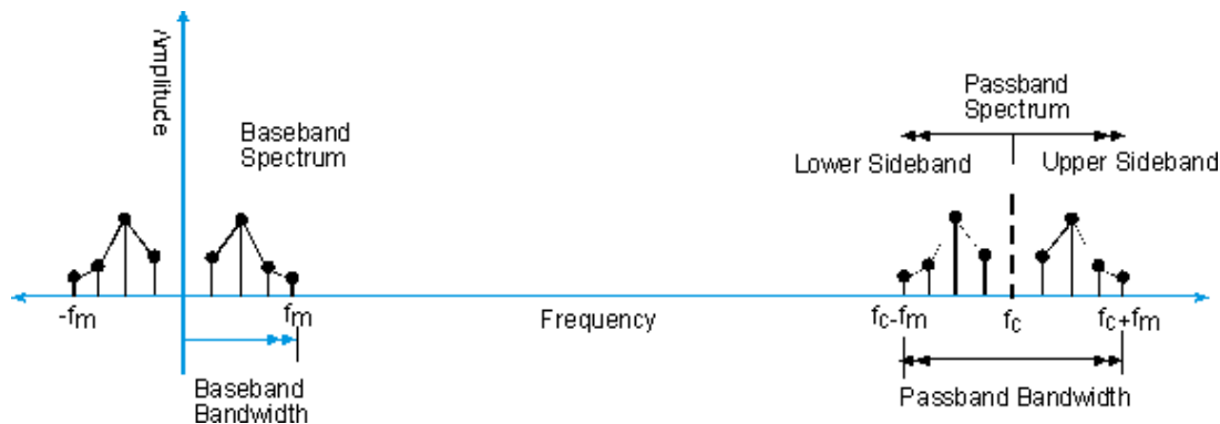
Figure 6 - Baseband becomes Passband by translation to higher frequency
