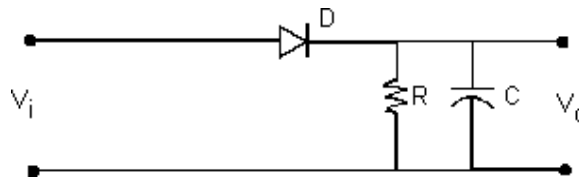
Figure 18 - RC-Diode Circuit used for Envelope Demodulation
